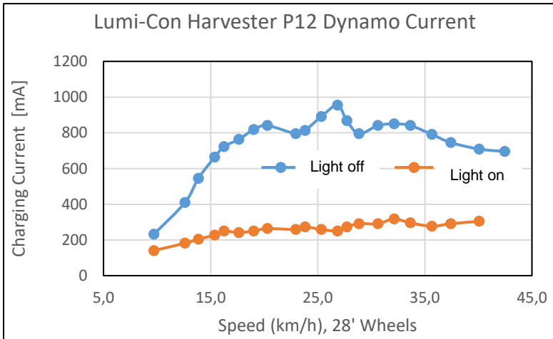
Fig. 3: Charge current vs. speed, for a typical hub dynamo (Shimano)
