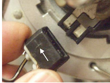
2) Disconnect and remember the wire which was connected to GND (symbol ⊥**)
