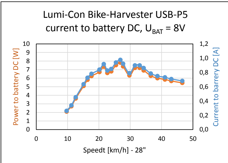
Fig. 3: Charge current and power at a battery voltage of 8V vs. speed, typical hub dynamo (Shimano)
