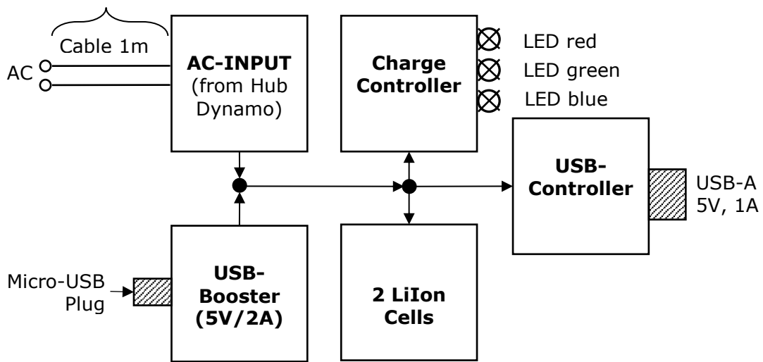
Fig 2: Harvester Functional Diagram
